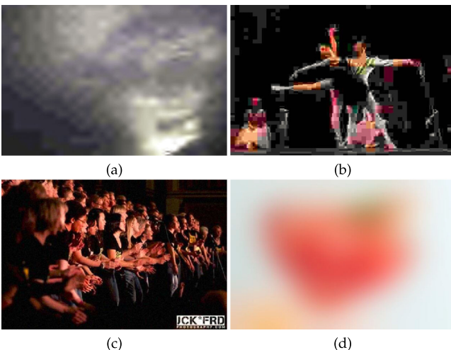
Fig. 4. gMAD image pairs between SSIM and MS-SSIM. Images (a)-(d) correspond to points A - D in Fig. 3. (a) MS-SSIM = 30, SSIM = 53. (b) MS-SSIM = 30, SSIM = 13. (c) SSIM = 30, MS-SSIM = 78. (d) SSIM = 30, MS-SSIM = 13.
