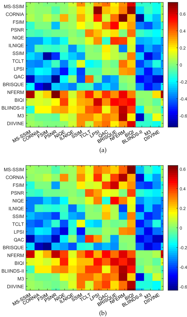
Fig. 6. Pairwise comparison results of the 16 IQA models. (a) Aggressiveness matrix. (b) Resistance matrix. Each entry indicates the aggressiveness/resistance of the row model against the column model. \mathbf{A} - \mathbf{A}^T and \mathbf{R} - \mathbf{R}^T are drawn here for better visibility.
