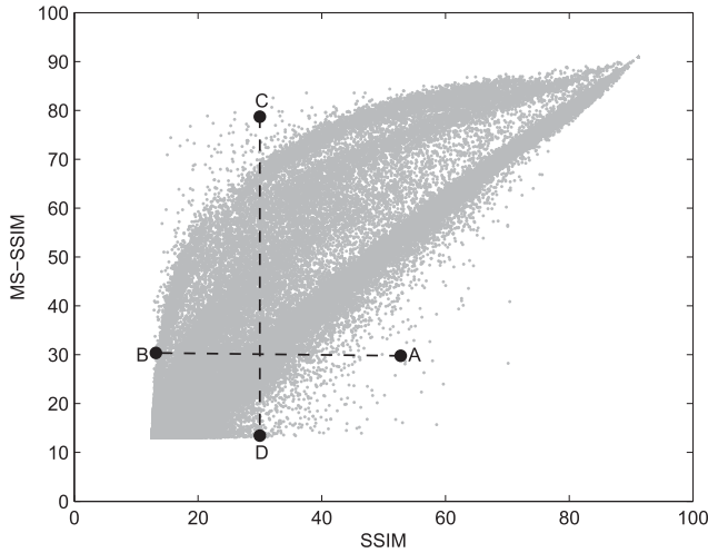
Fig. 3. gMAD image pairs from the Waterloo Exploration Database [19]. The image pair (A, B) is selected by maximizing/minimizing SSIM while holding MS-SSIM fixed. Similarly, (C, D) is selected by maximizing/minimizing MS-SSIM while holding SSIM fixed.
