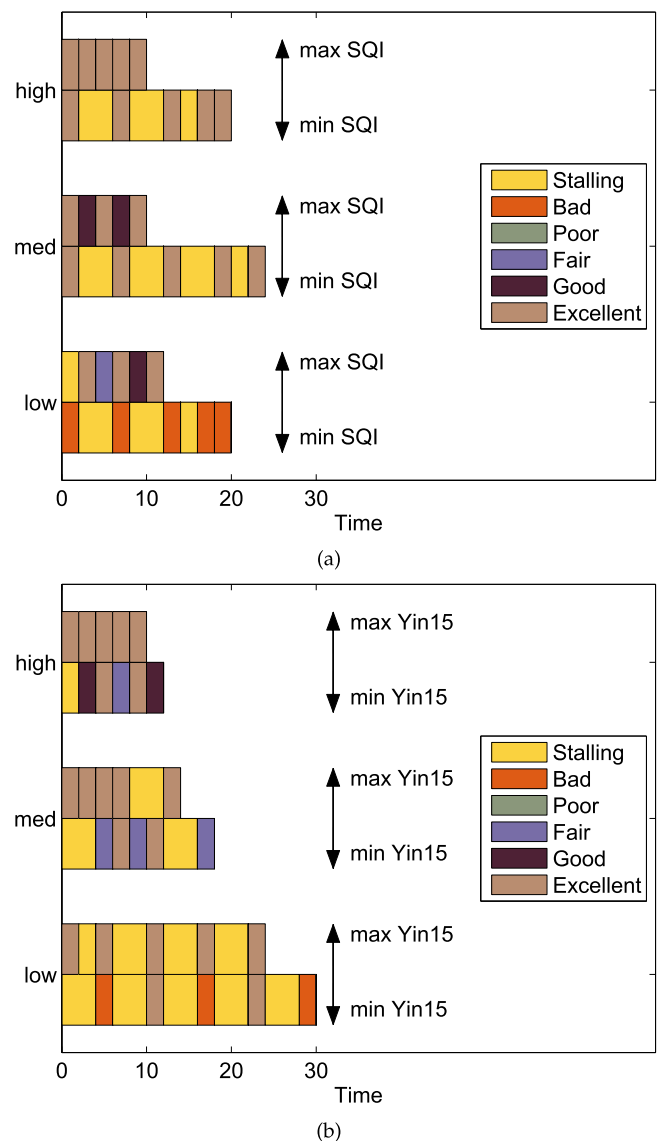
Fig. 11. gMAD competition between Yin15 [64] and SQI [58]. (a) Yin15 as defender. (b) SQI as defender. Video playout sequences at different video quality levels (as listed in Table 4) and the stalling events are represented using different color bars. The gMAD competitions are performed at high-, mid-, and low-QoE levels, respectively.
